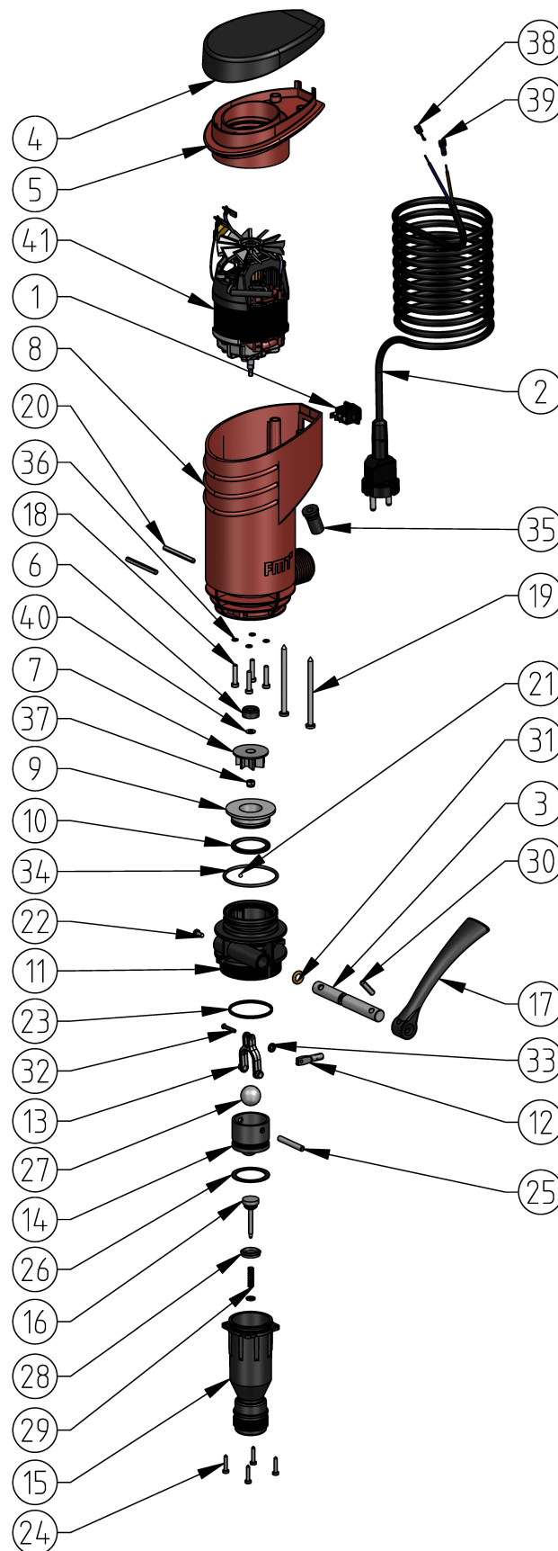
Fig. 13-1: Exploded view of the PREMAxx diesel pump 230 V
