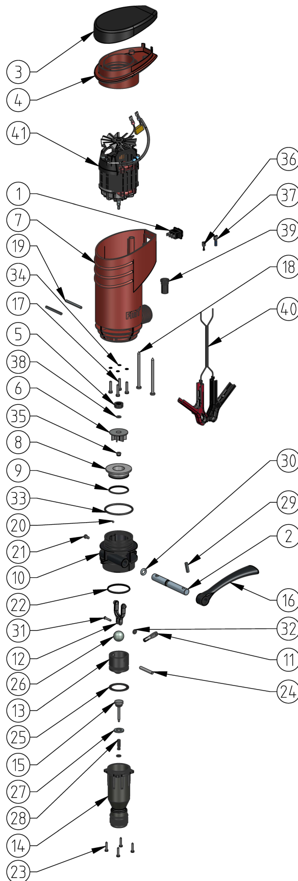
Fig. 14-1: Exploded view of the PREMAxx diesel pump 24 / 12 V
