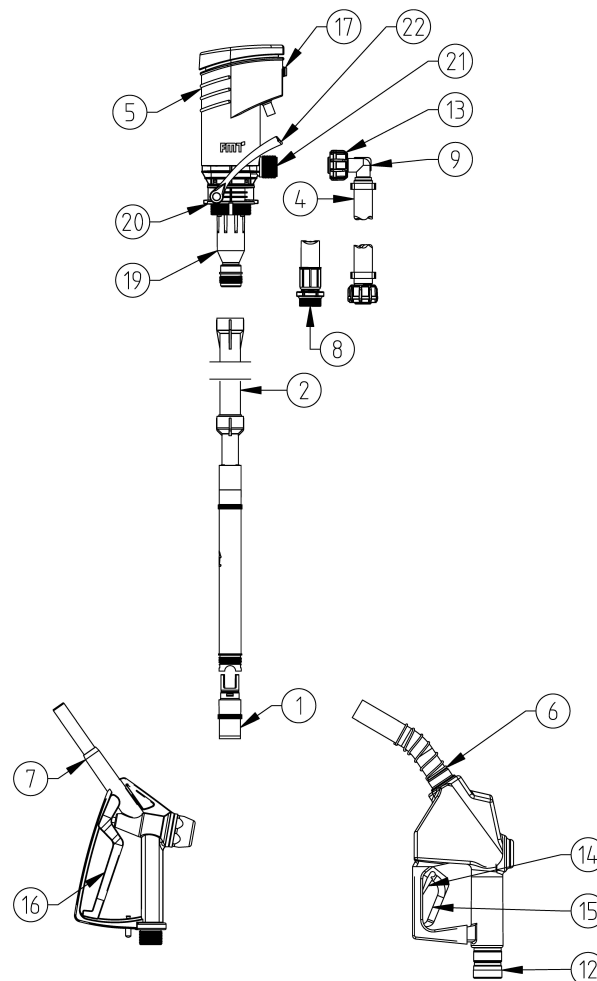
Fig. 6-1: Overview of the PREMAxx diesel pump with accessories
