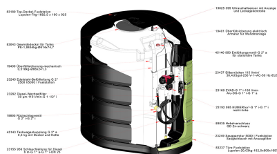
26760 Revision A Fuelstation-5000 I - 230 V-115 I-EBZM-F
